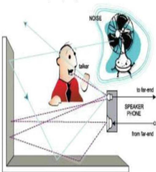
Fig 1: Acoustic Echo
